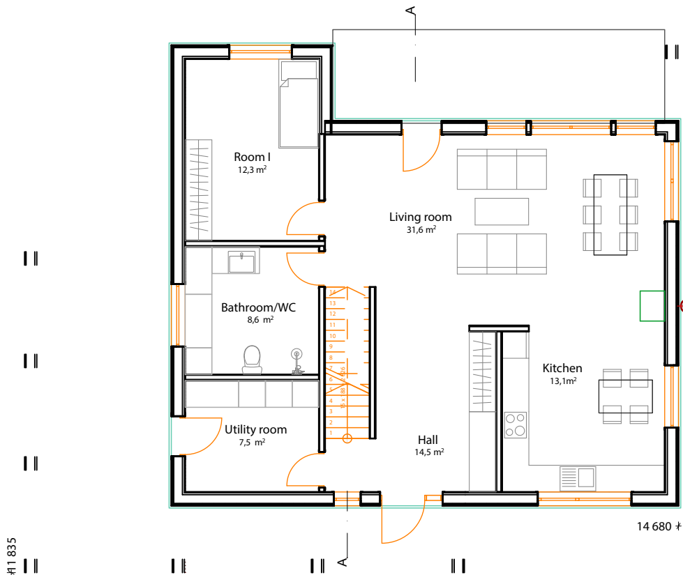
1st floor
